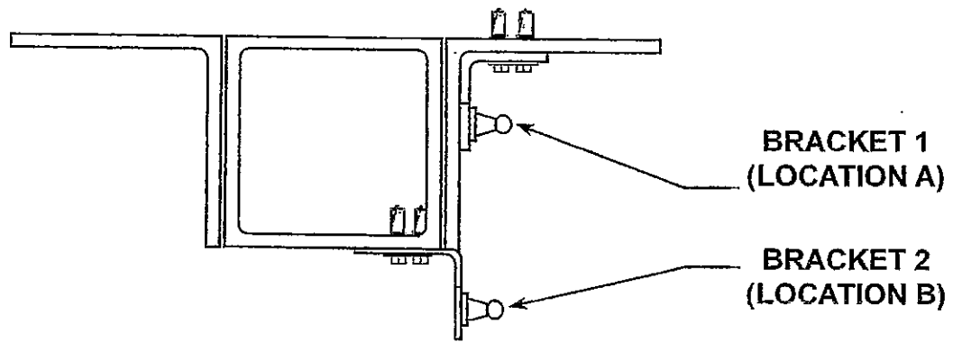
CLOSE-UP VIEW IN TOW POSITION (FRONT CUT-AWAY ANGLE)
